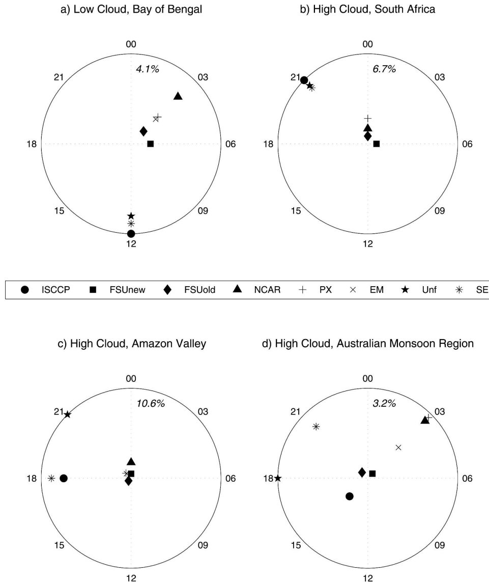
FIG. 12. Sundial representation of the phase and amplitude of the diurnal cycle of low and high clouds over (a) the Bay of Bengal ( 0^{\circ} – 20^{\circ} N, 80^{\circ} – 100^{\circ} E), (b) South Africa ( 35^{\circ} – 5^{\circ} S, 10^{\circ} – 40^{\circ} E), (c) Amazon valley ( 15^{\circ} – 5^{\circ} S, 60^{\circ} – 50^{\circ} W), and (d) Australian monsoon region ( 20^{\circ} S– 0^{\circ} , 120^{\circ} – 140^{\circ} E) from ISCCP and day-5 forecast of the four member models, their ensemble mean, the unified cloud scheme, and the SE during 22–31 Mar 2000. The representative amplitude of the radius of each dial is indicated by the number at the top (near 0 h) in percent.
