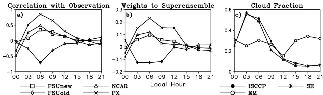
FIG. 2. Illustration of the performance of member models over a grid point (18°S, 133°E) for low cloud and the need to assign different weights to the member models based on their performance: (a) cross correlation of the model-simulated low cloud fraction with that of the ISCCP at each hour during the training period, (b) weights assigned to the member models at each hour to construct the SE, and (c) ISCCP satellite-based estimates of low cloud and predicted low cloud by the ensemble mean of the models and the SE. Legends are same for (a) and (b) and separate for (c).
