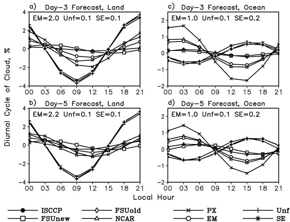
FIG. 8. Diurnal cycle of high cloud cover over the Tropics ( 30^{\circ}\text{S} – 30^{\circ}\text{N} , 0^{\circ} – 360^{\circ}\text{E} ) from ISCCP and day 3 and 5 of forecasts from the member models, EM, Unified, and SE during 22–31 Mar 2000. The rms errors (%) of the total diurnal cycle for EM, Unified, and SE are indicated at the top of each panel.
