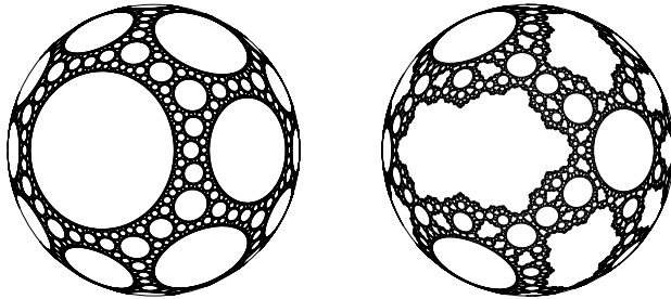
FIGURE 2. Non-trivial quasiconformal deformation 2
