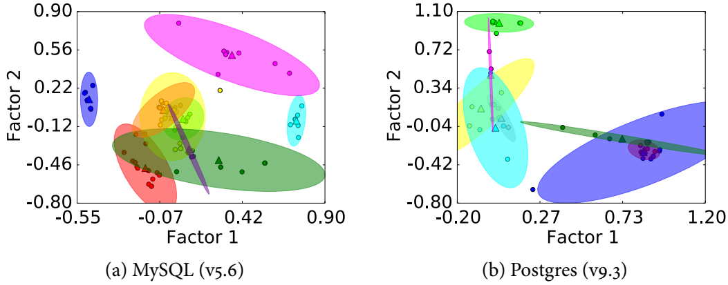
Figure 3.2: Metric Clustering – Grouping DBMS metrics using k -means based on how similar they are to each other as identified by Factor Analysis and plotted by their (f1, f2) coordinates. The color of each metric shows its cluster membership. The triangles represent the cluster centers.
