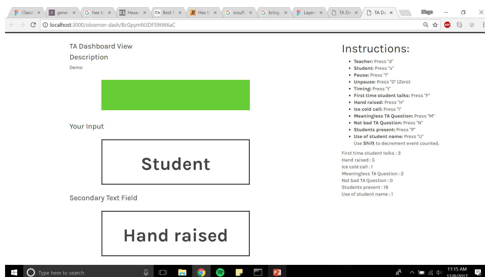
Figure 4.1: User interface of the TA Dashboard.
