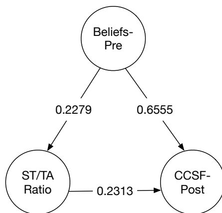
Figure 7.13: Simple Latent variable model of pretest measures of belief, Student talk, and student-focus post-test with the relevant path coefficients ( all TAs ).
