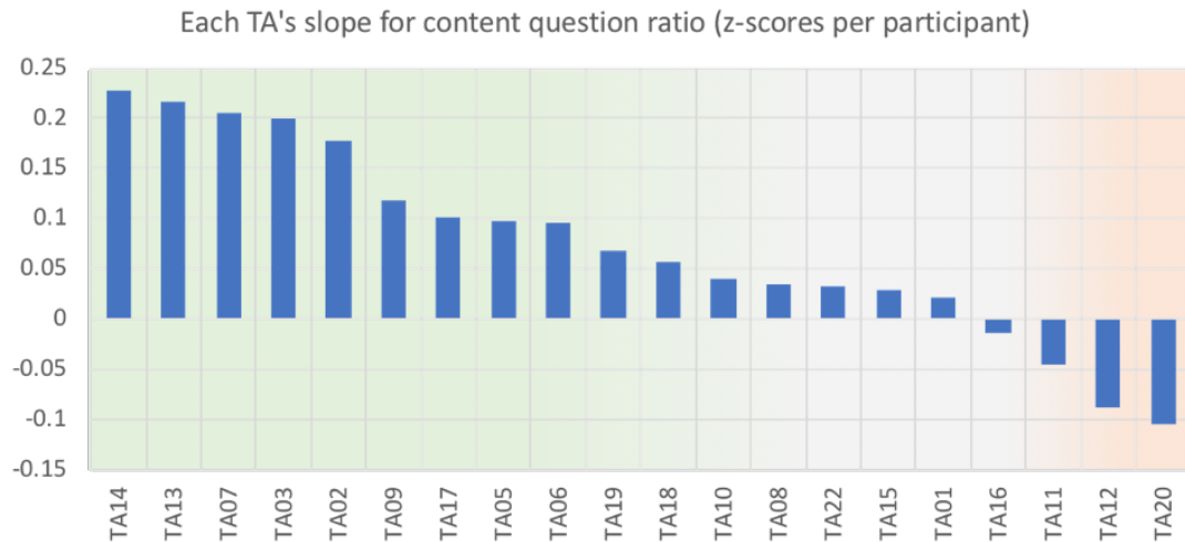
Figure 7.6: (Pg. 92) Example raw values for the content question ratio variable for three participants across teaching opportunities, and (above) their corresponding z-scores in context of all participants. Participants in the green section of the graph are categorized as improvement for this variable, white represents no change, and orange indicates decline.
