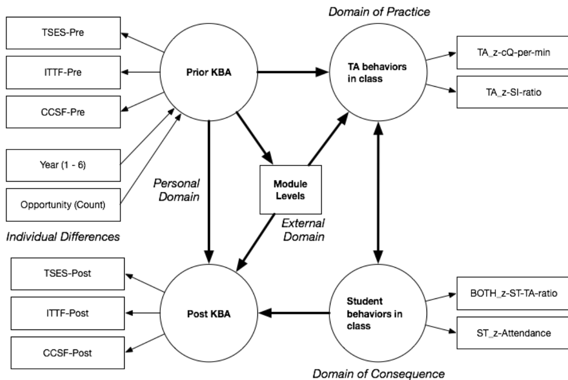
Figure 7.14: Confirmatory model of the PAR-TS Framework based on Study 4 data.
