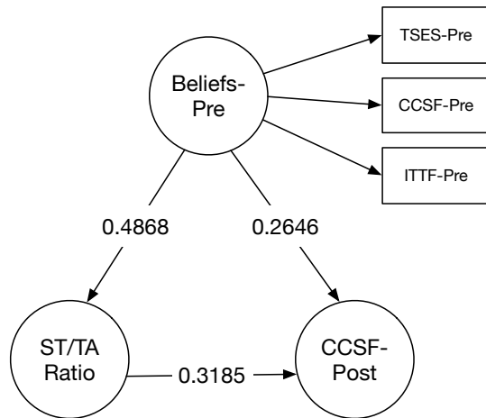
Figure 7.12: Simple Latent variable model of pretest measures of belief, Student talk, and student-focus post-test with the relevant path coefficients ( B_Group only).
