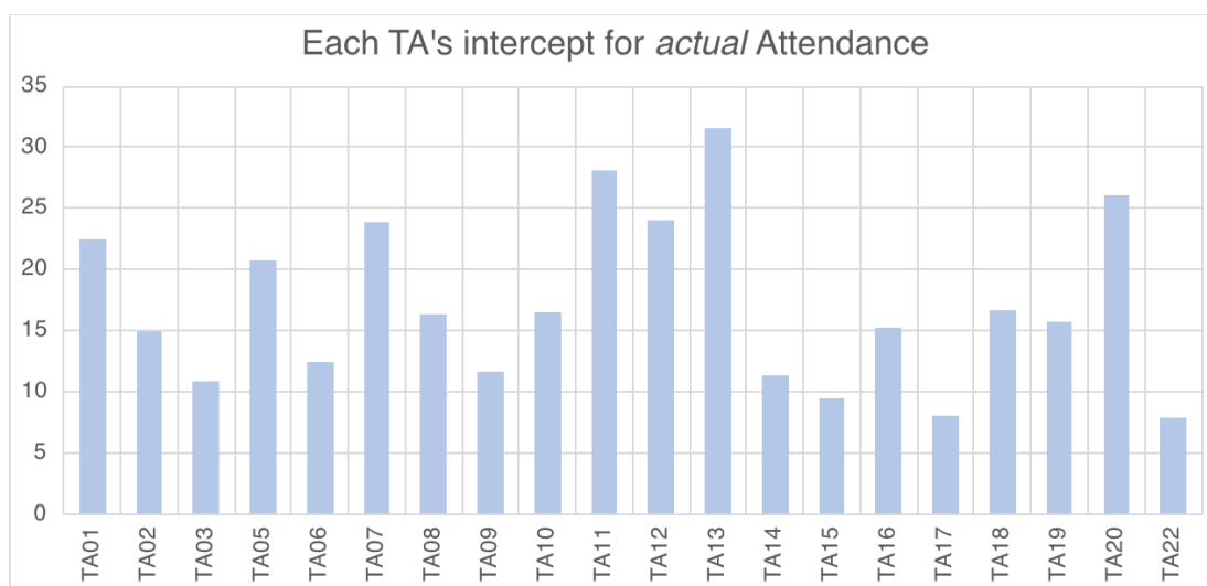
Figure 7.9: Calculated intercept for actual number of students in attendance (y-axis) for each TA.
